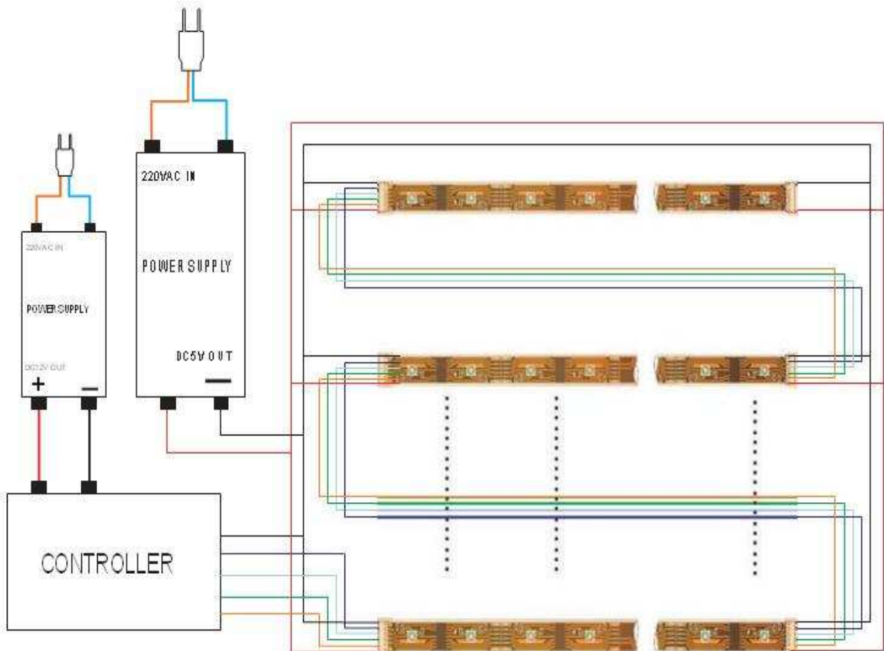
Wiring Diagram
