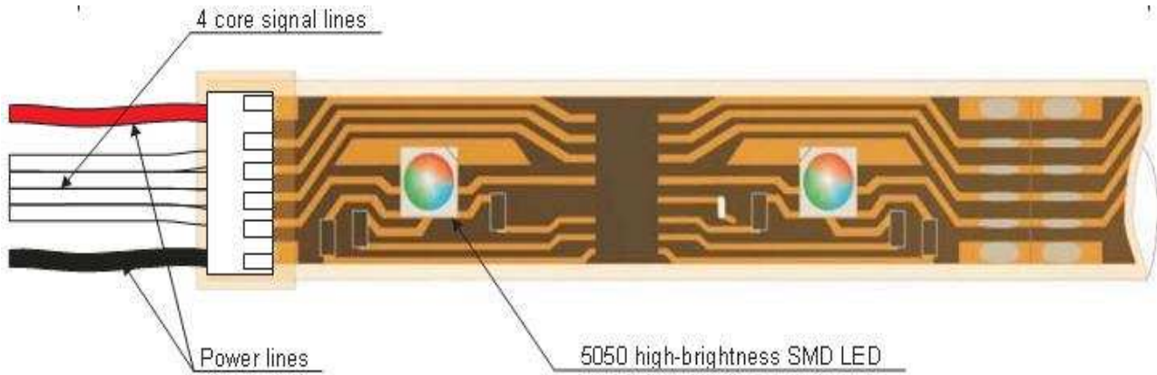
Wiring Diagram
