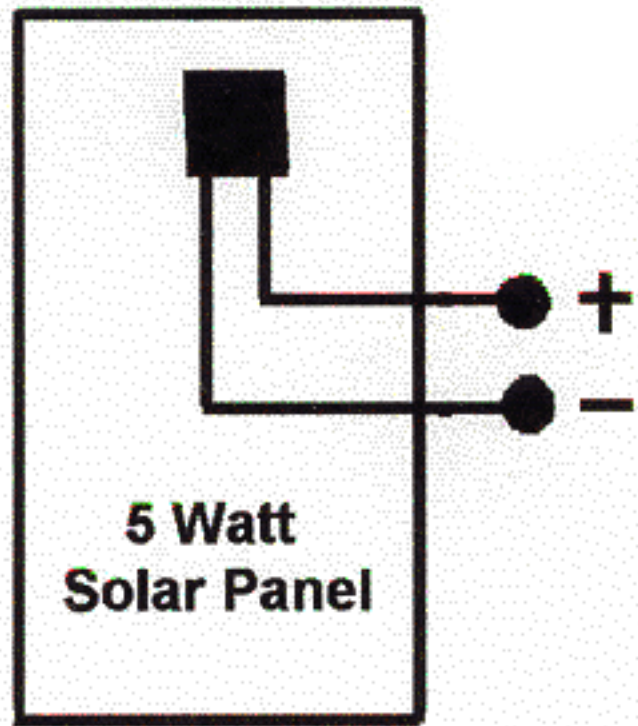
5 Watt Solar Panel 12 VDC at 400 ma
