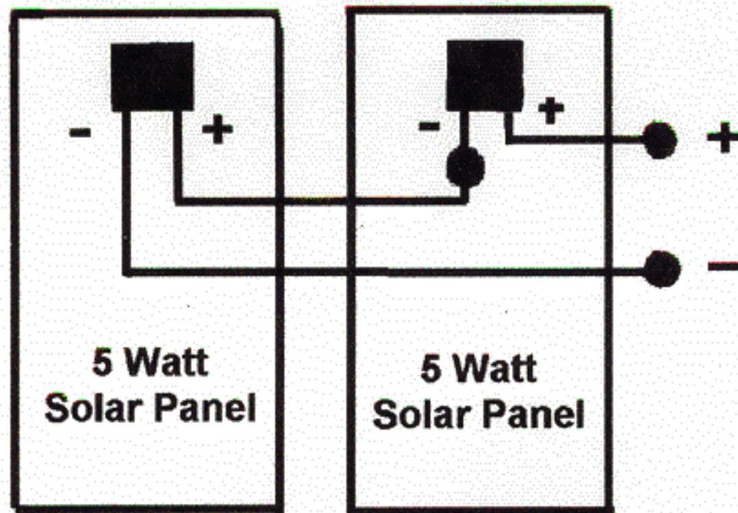
Two 5 Watt Solar Panels Connected in SERIES Gives You 24 VDC at 400 ma at 10 Watts
