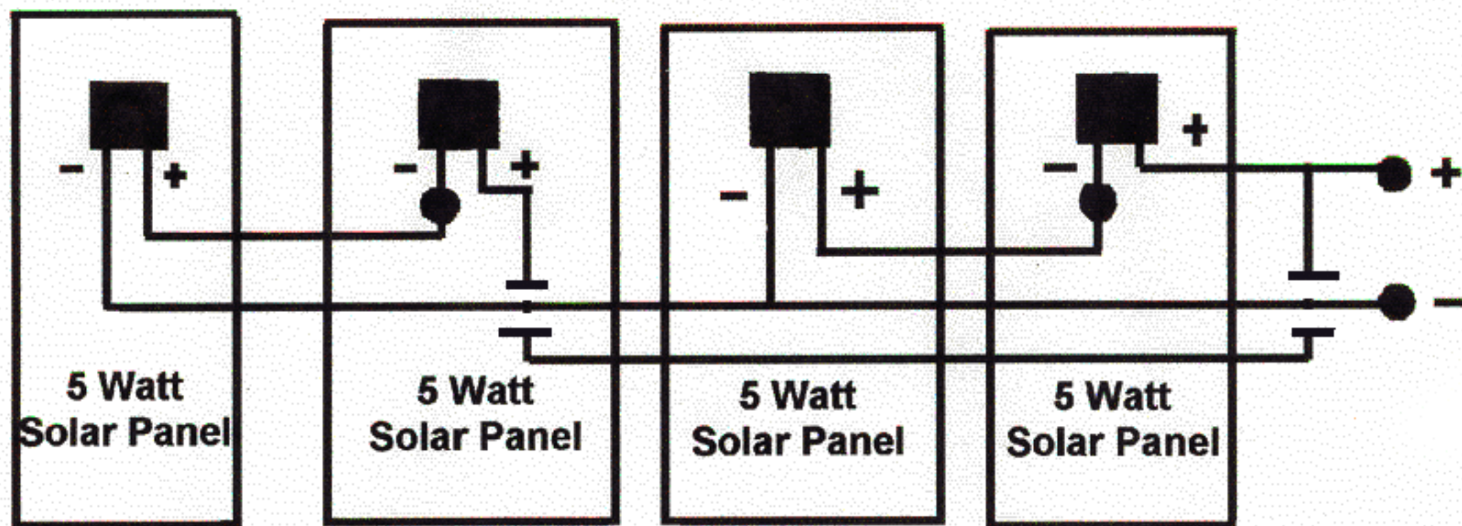
Four 5 Watt Solar Panels Connected in SERIES PARALLEL Gives You 24 VDC at 800 ma at 20 Watts
