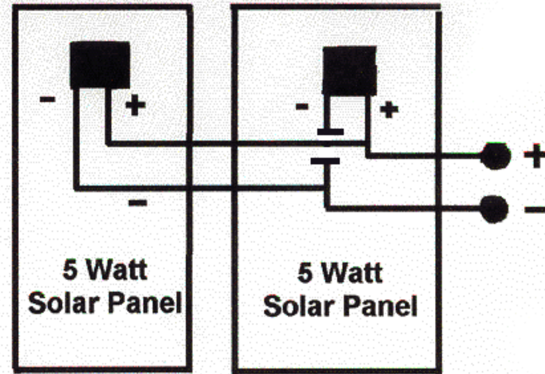
Two 5 Watt Solar Panels Hooked in PARALLEL Equal 10 Watts at 12 VDC 800 ma at 10 Watts
