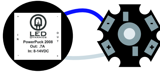
700mA PowerPuck Driving a 5W Luxeon
