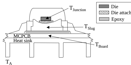
Figure 1B. Emitter Cut-Away
