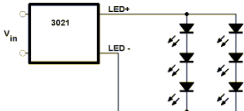
Figure 3. 700mA unit driving Lumileds 6-ring ( V_{IN} \geq 12VDC )
