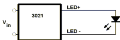
Figure 7. 700mA unit driving one Luxeon® V emitter ( V_{in} \geq 12VDC )
