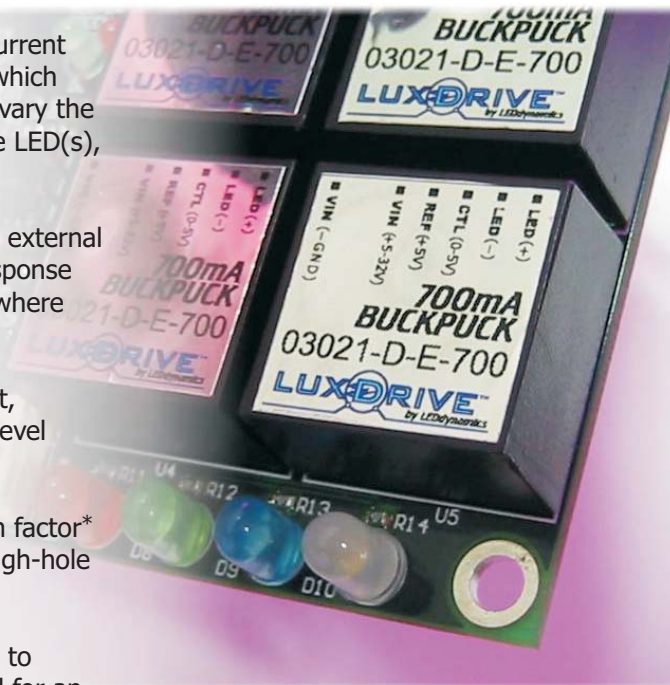
(4) 03021-D-E-700 BUCKPUCKs mounted to LuxDrive's 4016 QuadPuck 4-Channel DMX Driver Interface
